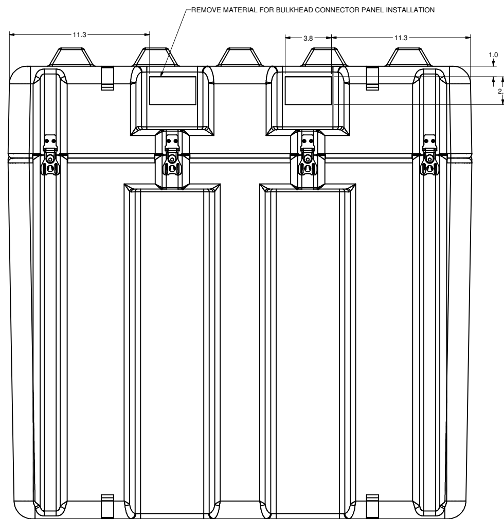
HARDIGG AL3434-2807 REAR VIEW
